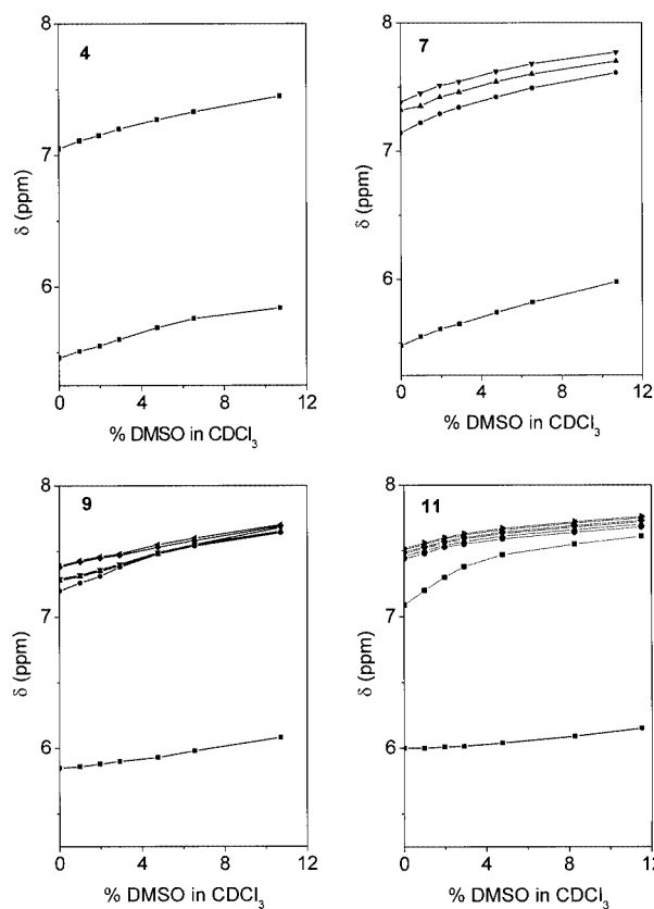
Figure 5. Plot of NH chemical shifts in the 1 H NMR spectra of oligomers Boc-( g Gly- m Aib) n -OBn 4 , 7 , 9 and 11 as a function of increasing percentages of DMSO added to the CDCl 3 solution (v/v); peptide concentration: 1 mM for 4 , 7 , and 9 ; 0.1 mM for 11
