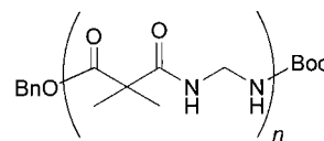
Figure 2. Chemical structure of the sequential Boc( g Gly- m Aib) n -OBn ( n = 1–4; 4, 7, 9, 11) peptide oligomers
